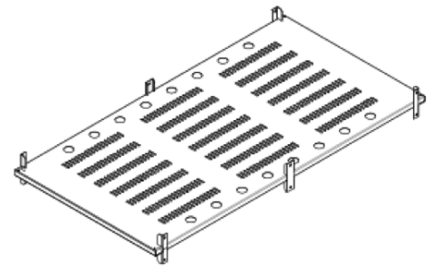
Vented Divider Panel
